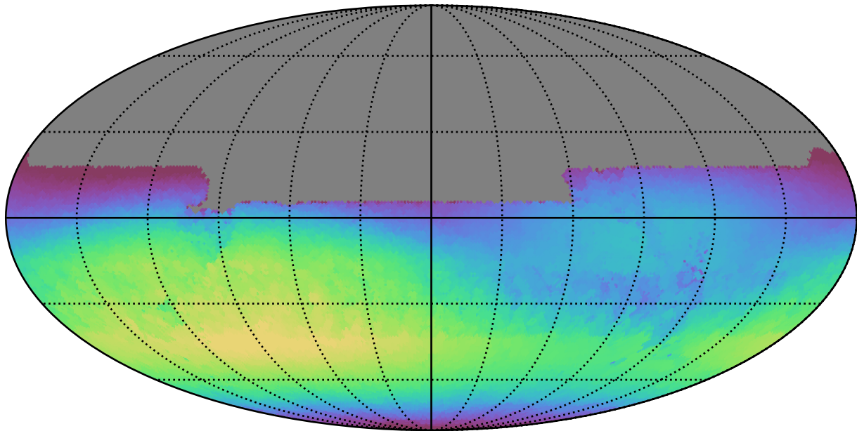
early_u_fpextra4.0_v3.4_10yrs All sky u band: Max skyBrightness
