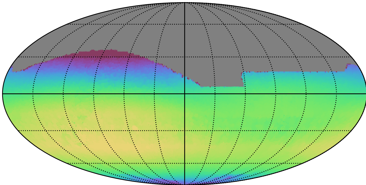
early_u_fpextra4.0_v3.4_10yrs All sky i band: Max skyBrightness
