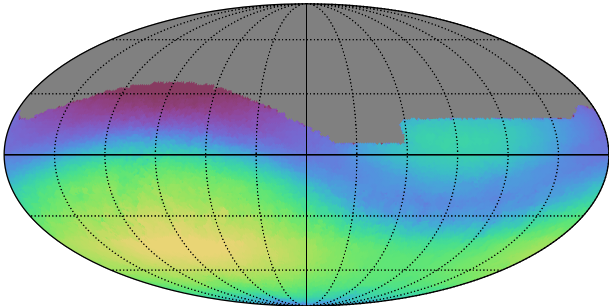
early_u_fpextra4.0_v3.4_10yrs All sky g band: Max skyBrightness
