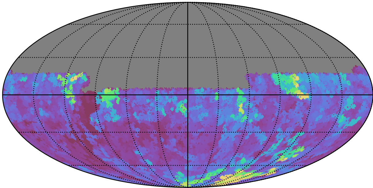
early_u_fpextra4.0_v3.4_10yrs Yr 1 u band: Max seeingGeom
