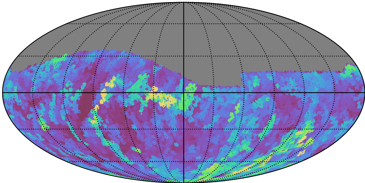
early_u_fpextra4.0_v3.4_10yrs Yr 1 r band: Max seeingGeom
