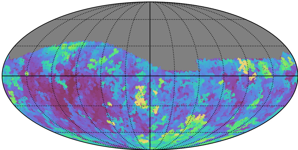
early_u_fpextra4.0_v3.4_10yrs Yr 1 g band: Max seeingGeom
