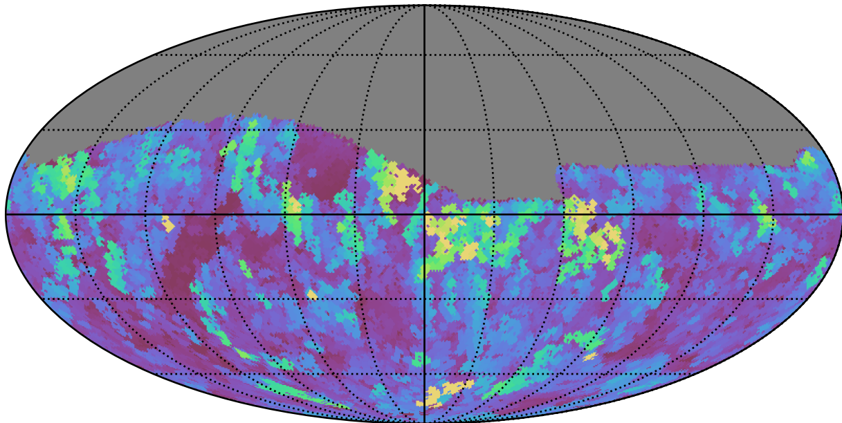
early_u_fpextra4.0_v3.4_10yrs Yr 1 z band: Max seeingEff
