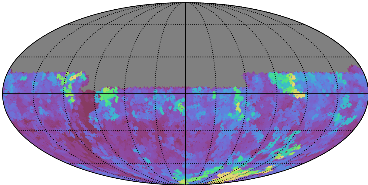
early_u_fpextra4.0_v3.4_10yrs Yr 1 u band: Max seeingEff
