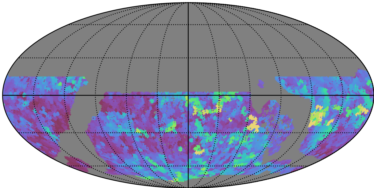
early_u_fpextra4.0_v3.4_10yrs WFD y band: Max seeingEff
