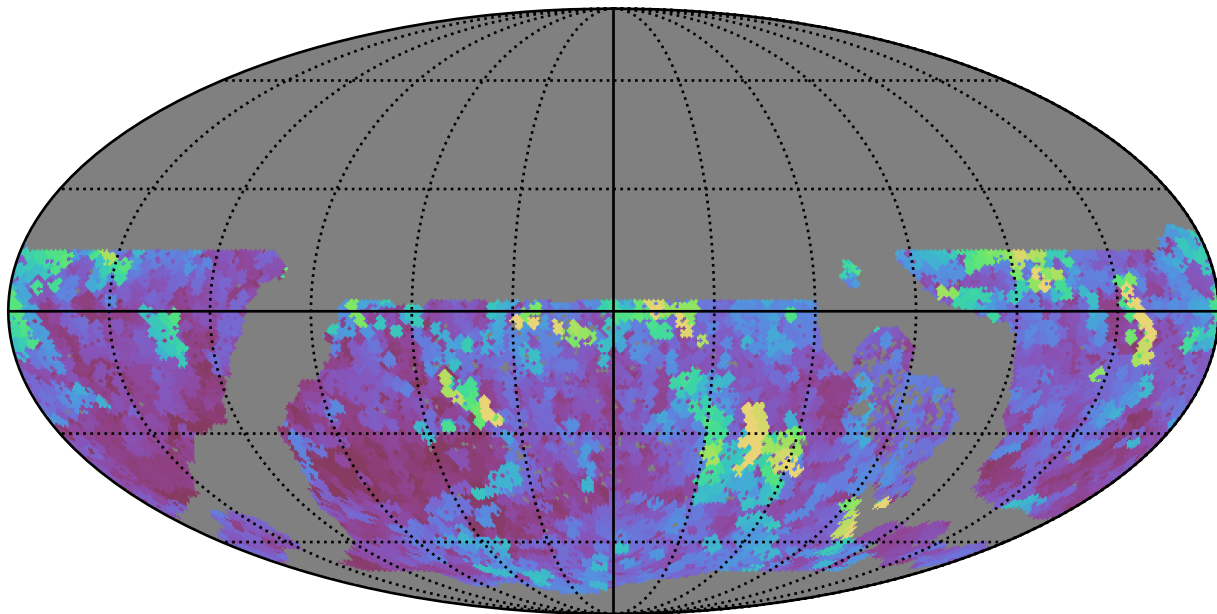
early_u_fpextra4.0_v3.4_10yrs WFD i band: Max seeingEff
