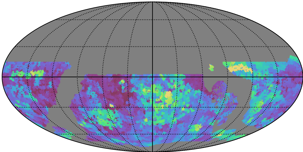
early_u_fpextra4.0_v3.4_10yrs WFD g band: Max seeingEff
