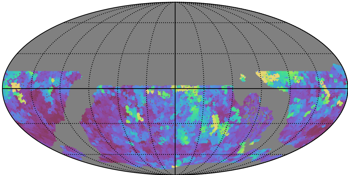
early_u_fpextra4.0_v3.4_10yrs WFD all bands: Max seeingEff
