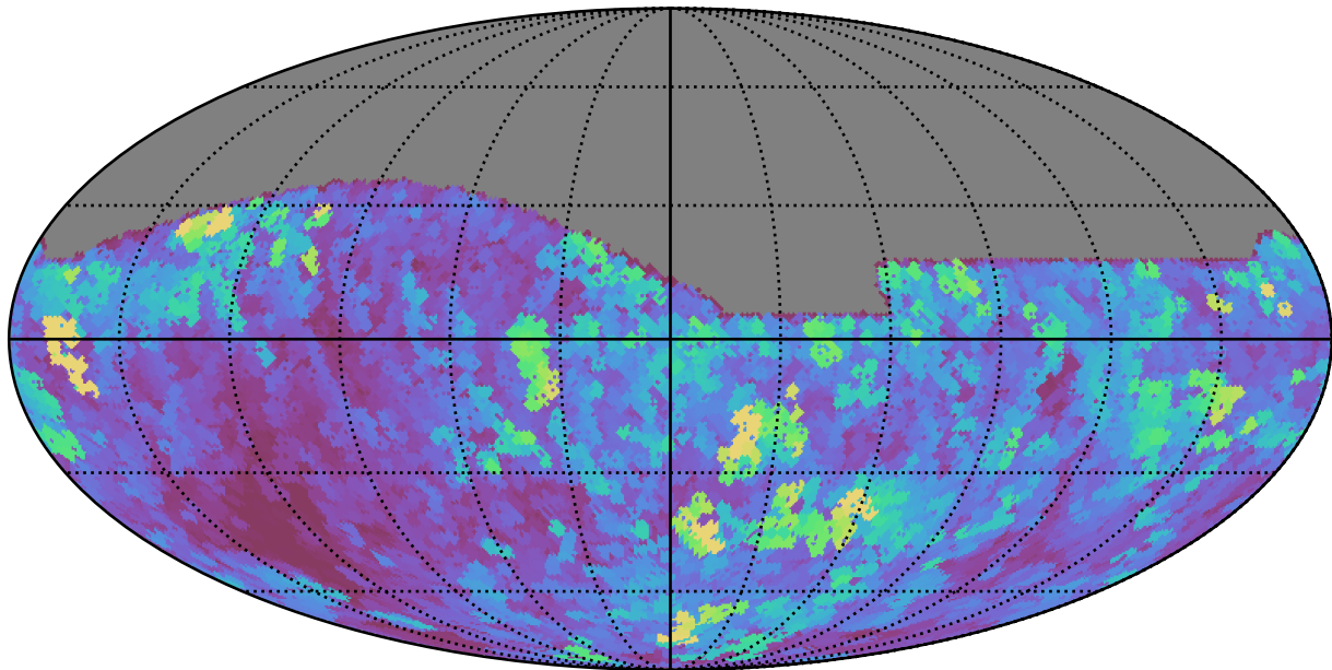
early_u_fpextra4.0_v3.4_10yrs All sky z band: Max seeingEff
