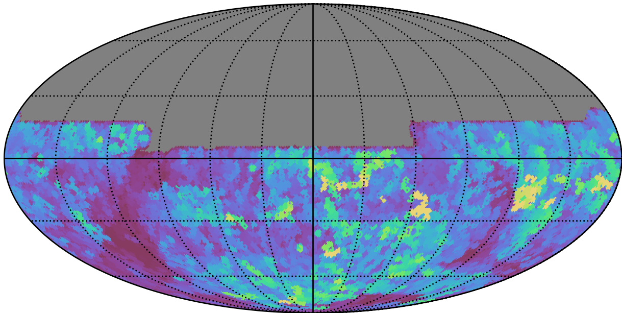
early_u_fpextra4.0_v3.4_10yrs All sky y band: Max seeingEff
