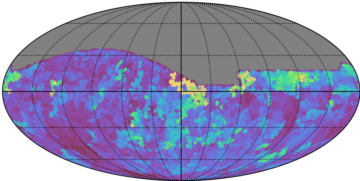
early_u_fpextra4.0_v3.4_10yrs All sky r band: Max seeingEff
