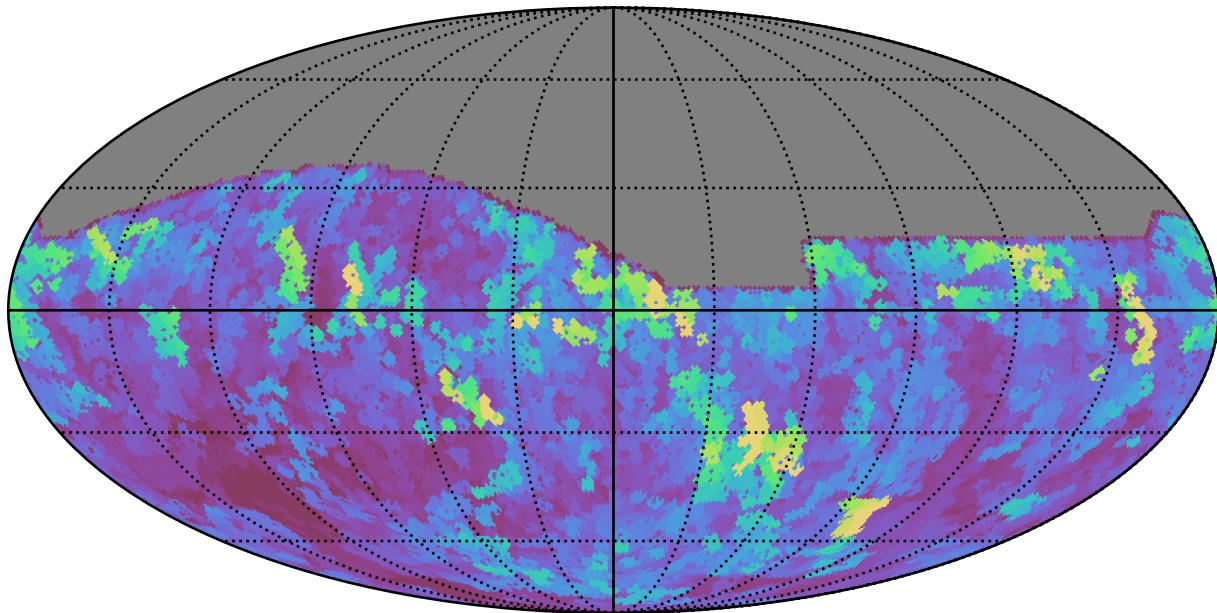
early_u_fpextra4.0_v3.4_10yrs All sky i band: Max seeingEff
