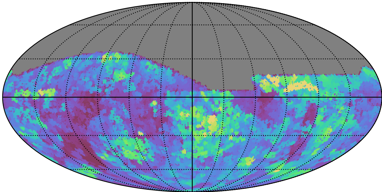
early_u_fpextra4.0_v3.4_10yrs All sky g band: Max seeingEff
