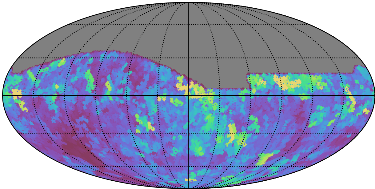
early_u_fpextra4.0_v3.4_10yrs All sky all bands: Max seeingEff
