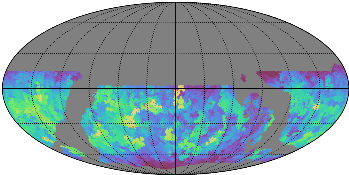
early_u_fpextra4.0_v3.4_10yrs WFD u band: Max saturation_mag
