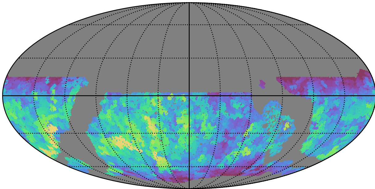
early_u_fpextra4.0_v3.4_10yrs WFD i band: Max saturation_mag
