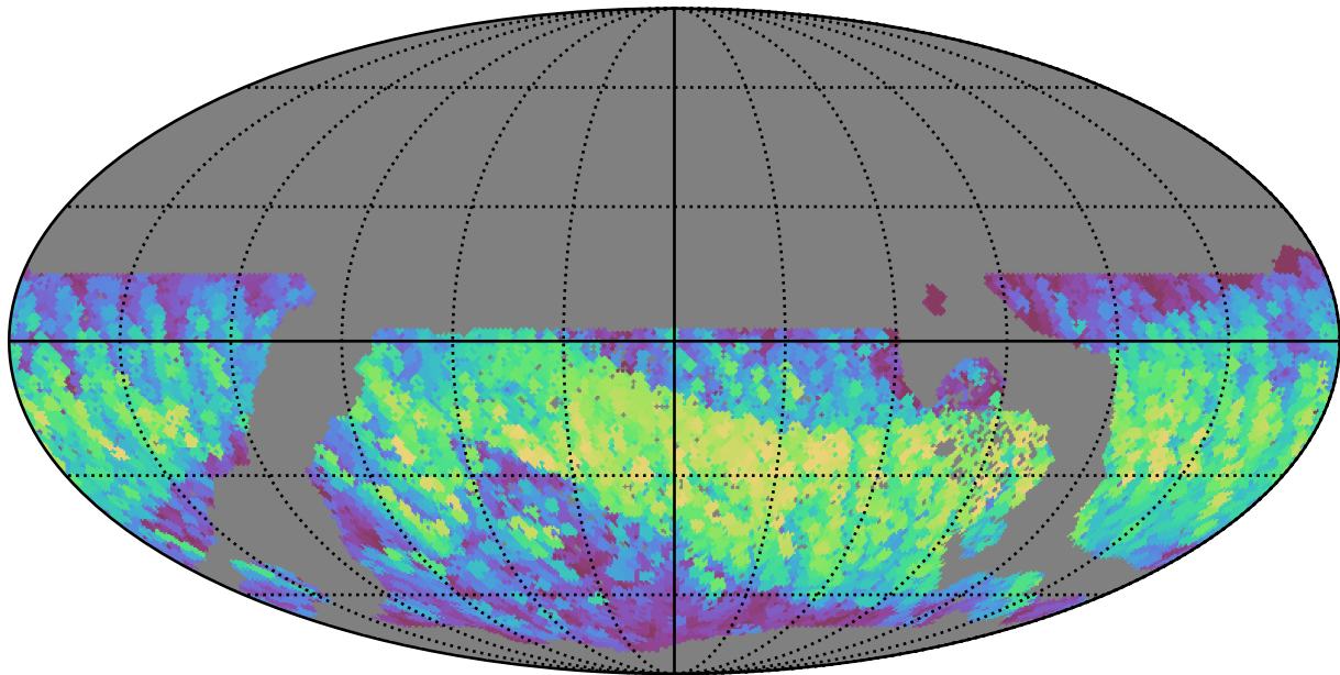
early_u_fpextra4.0_v3.4_10yrs WFD z band: Max normairmass
