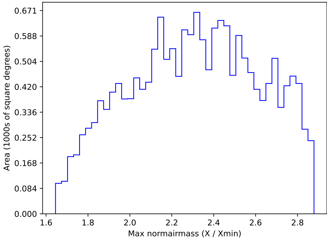
early_u_fpextra4.0_v3.4_10yrs WFD z band: Max normairmass
