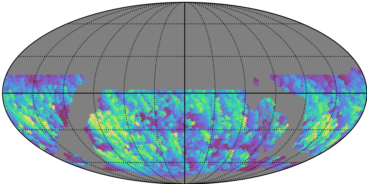
early_u_fpextra4.0_v3.4_10yrs WFD y band: Max normairmass
