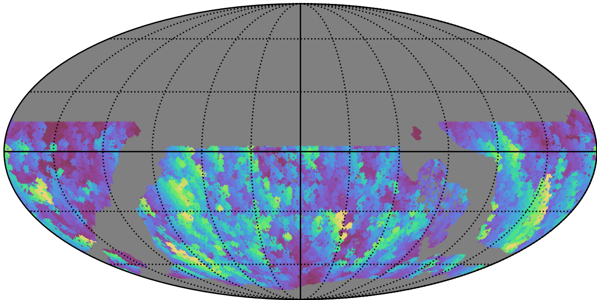
early_u_fpextra4.0_v3.4_10yrs WFD u band: Max normairmass
