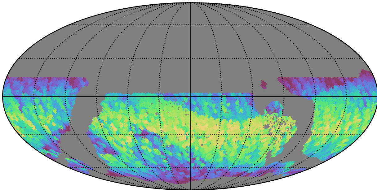
early_u_fpextra4.0_v3.4_10yrs WFD all bands: Max normairmass
