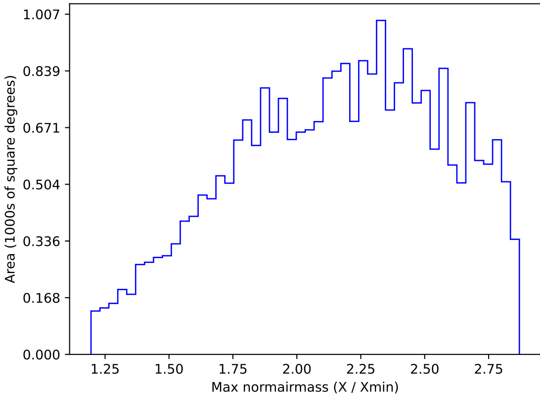
early_u_fpextra4.0_v3.4_10yrs All sky z band: Max normairmass
