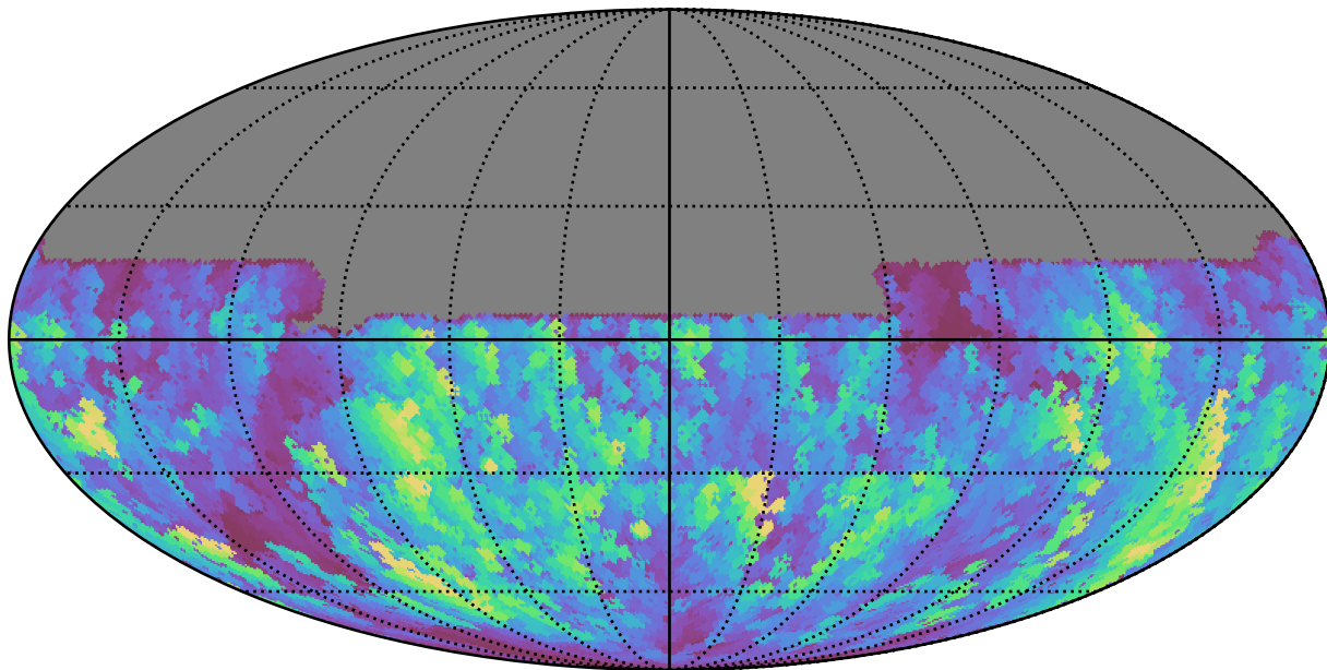
early_u_fpextra4.0_v3.4_10yrs All sky u band: Max normairmass
