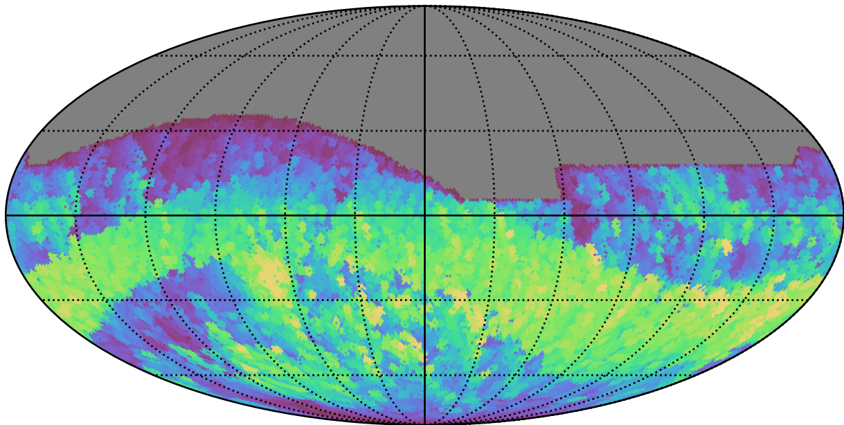
early_u_fpextra4.0_v3.4_10yrs All sky r band: Max normairmass
