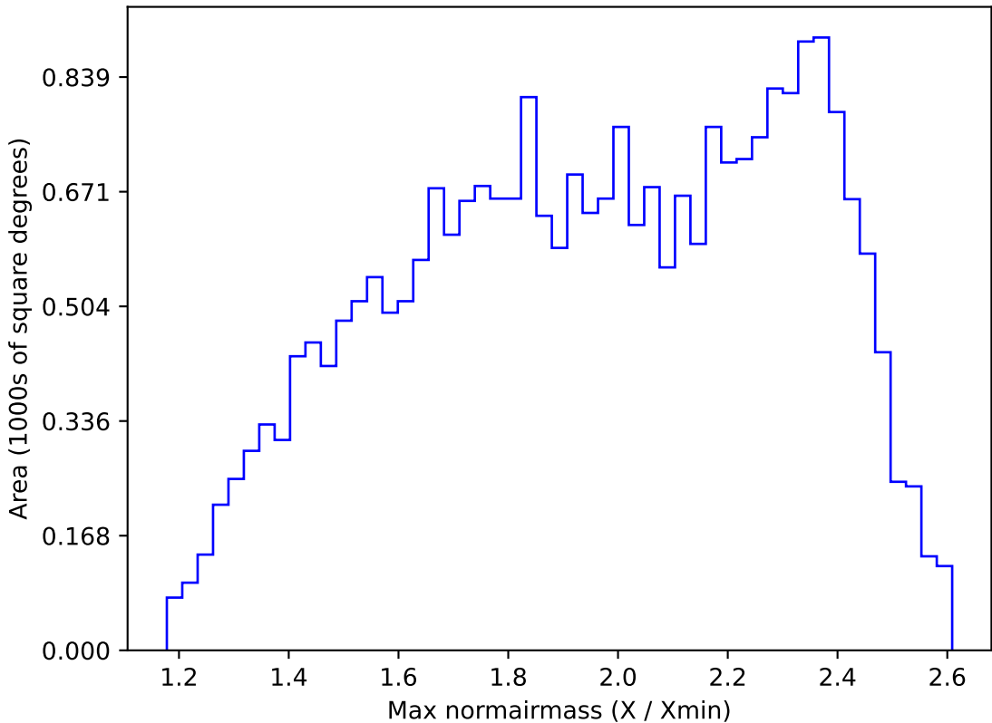
early_u_fpextra4.0_v3.4_10yrs All sky r band: Max normairmass
