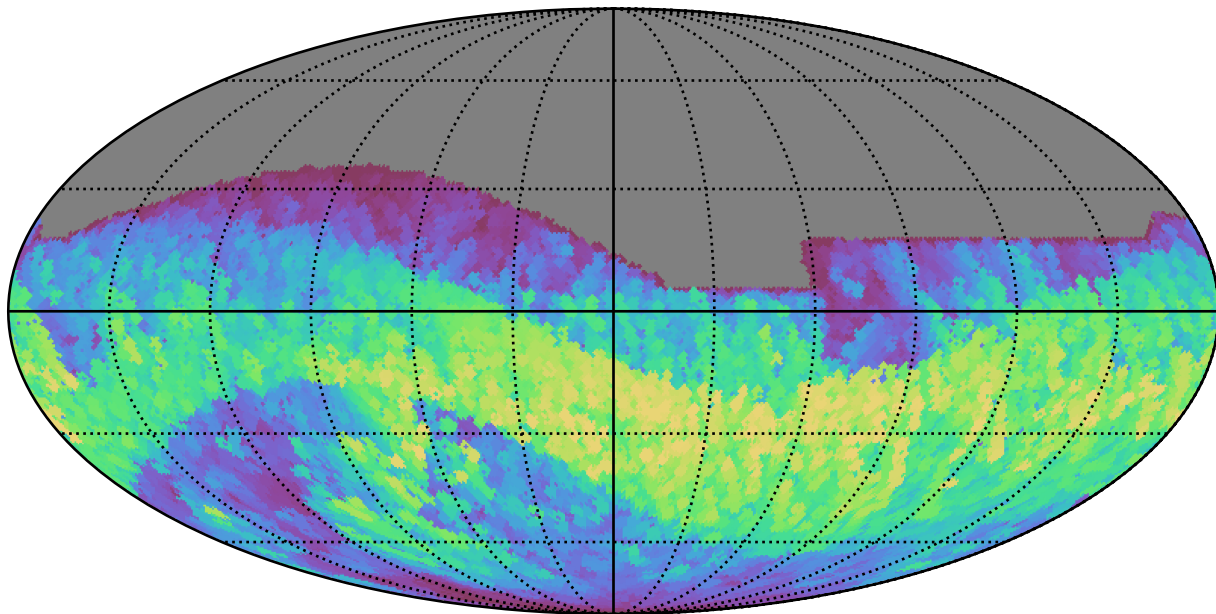
early_u_fpextra4.0_v3.4_10yrs All sky i band: Max normairmass
