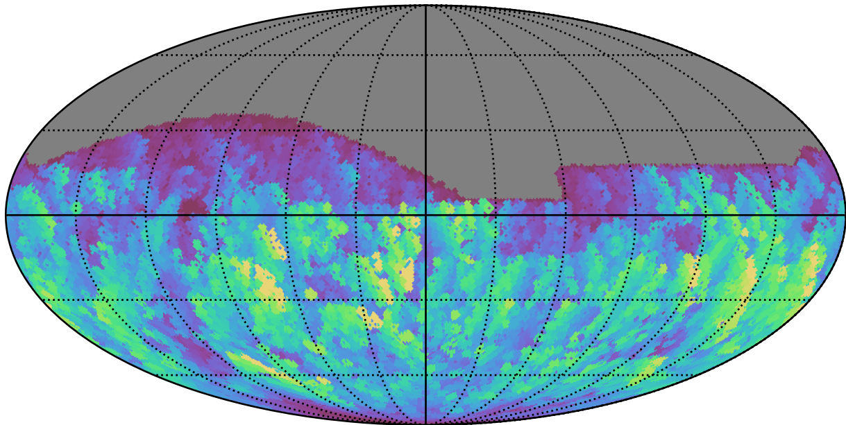
early_u_fpextra4.0_v3.4_10yrs All sky g band: Max normairmass
