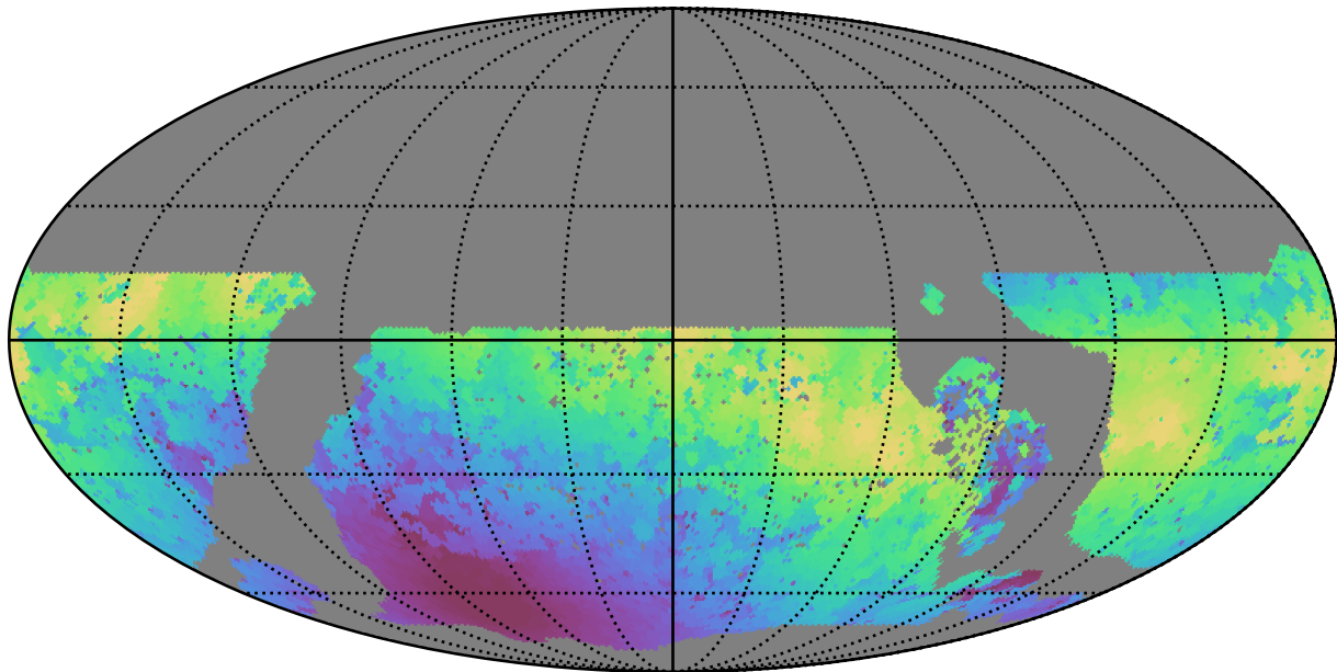
early_u_fpextra4.0_v3.4_10yrs WFD y band: Max moonDistance
