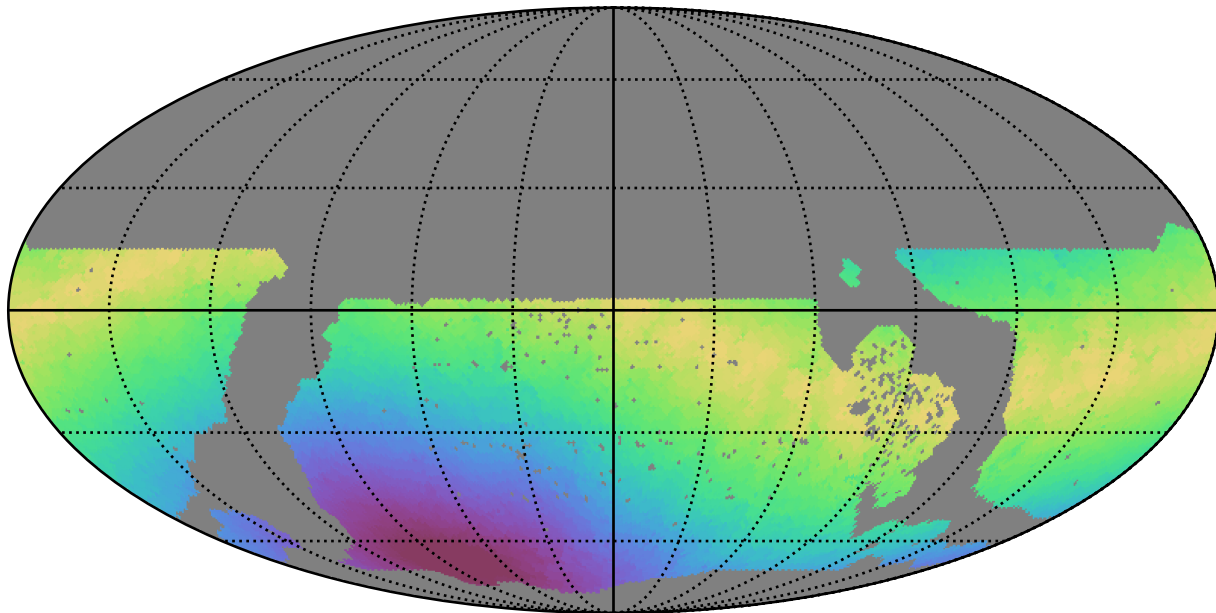
early_u_fpextra4.0_v3.4_10yrs WFD g band: Max moonDistance
