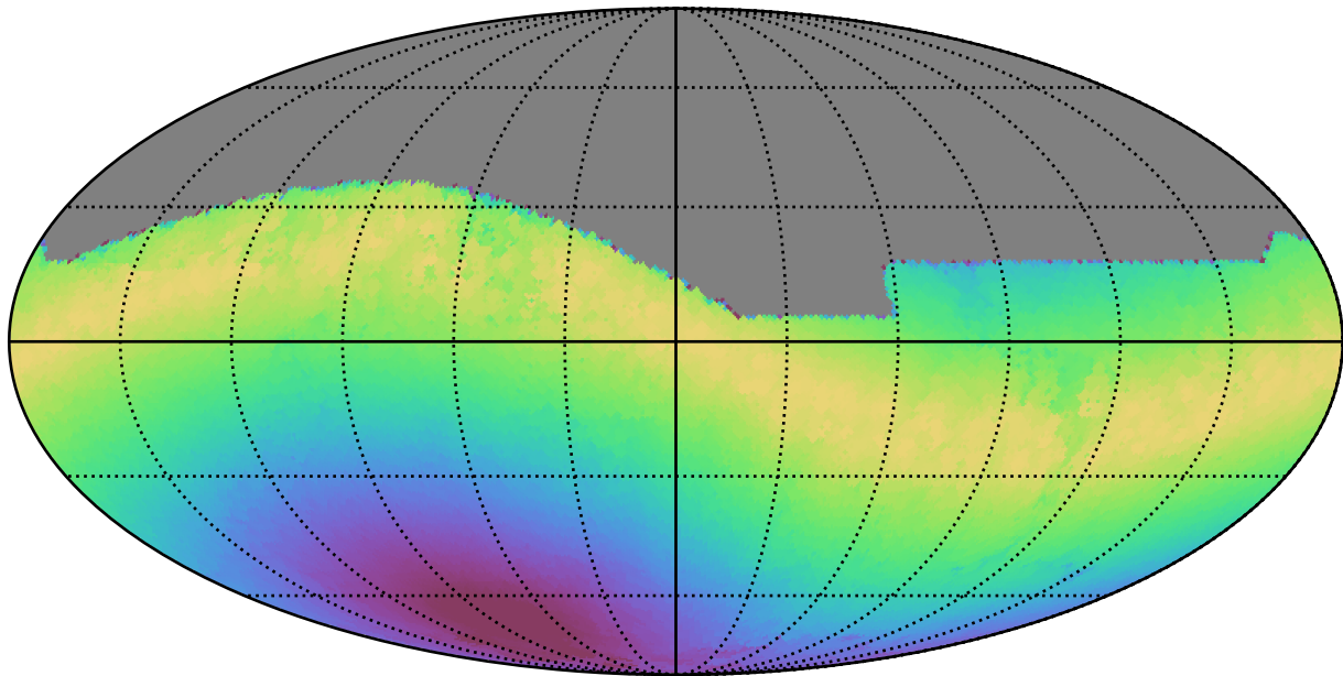
early_u_fpextra4.0_v3.4_10yrs All sky r band: Max moonDistance
