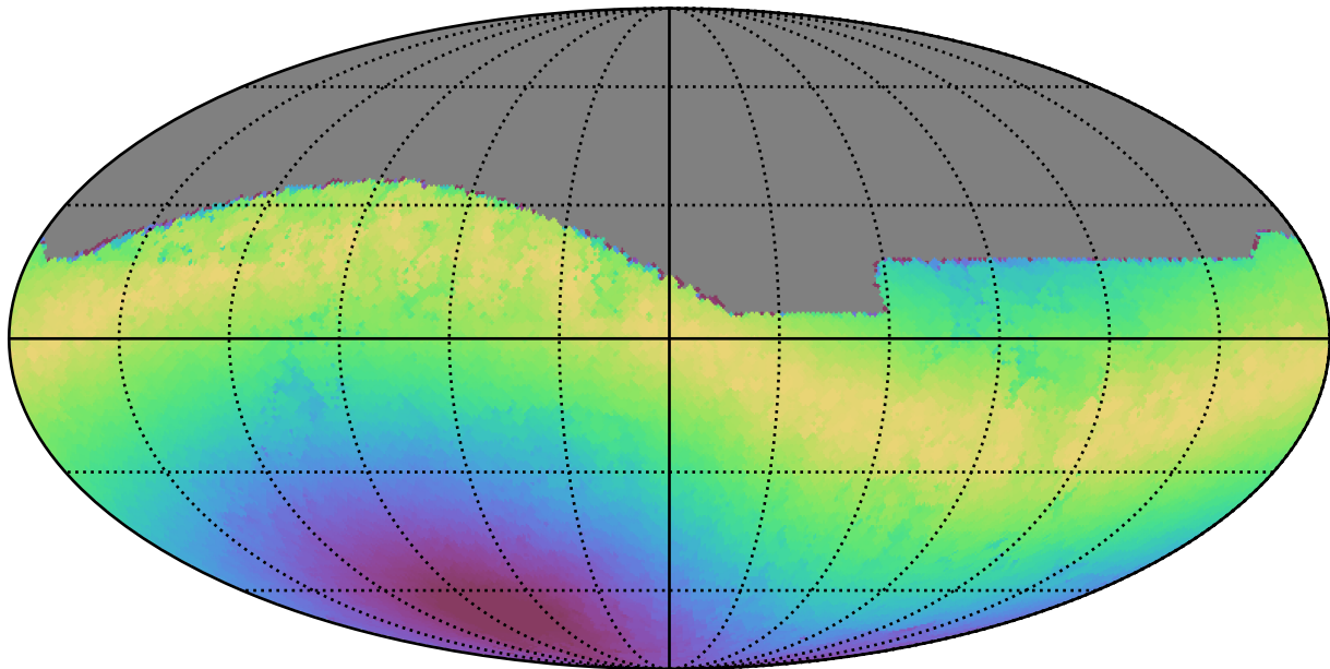
early_u_fpextra4.0_v3.4_10yrs All sky i band: Max moonDistance
