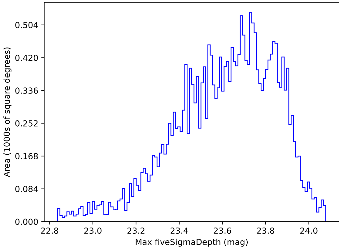
early_u_fpextra4.0_v3.4_10yrs Yr 1 u band: Max fiveSigmaDepth
