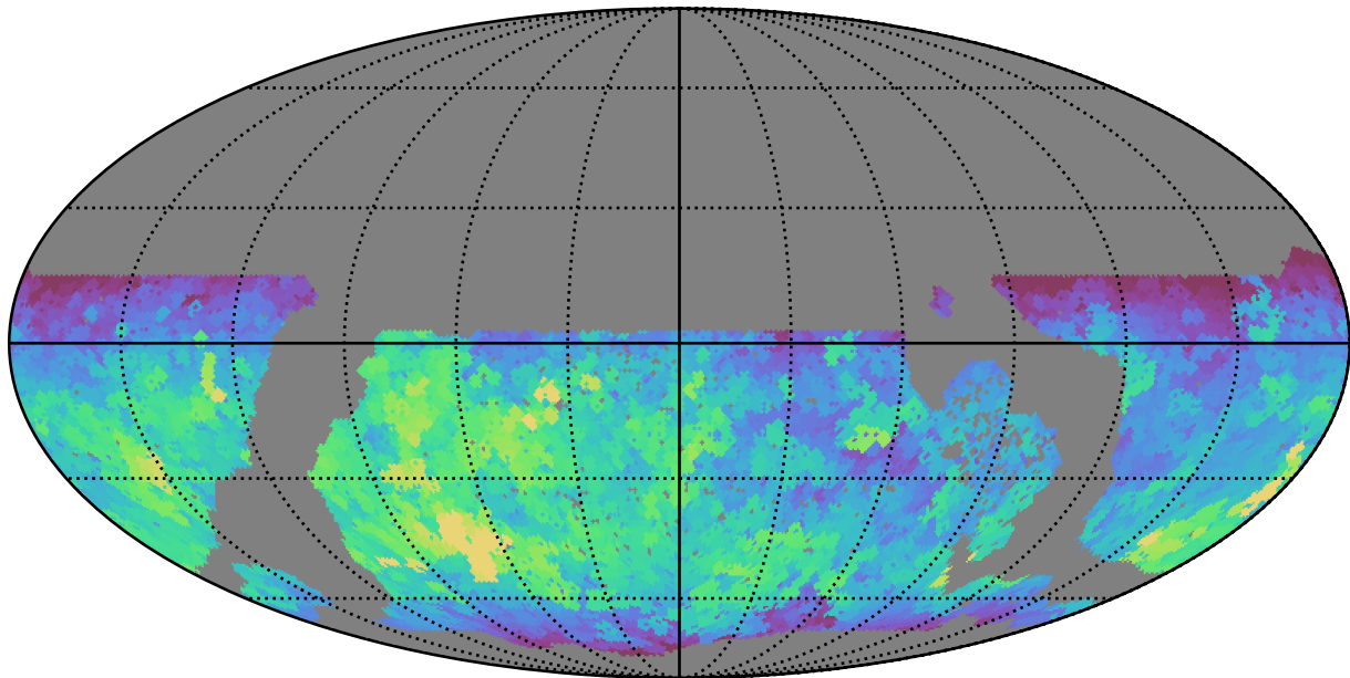
early_u_fpextra4.0_v3.4_10yrs WFD r band: Max fiveSigmaDepth
