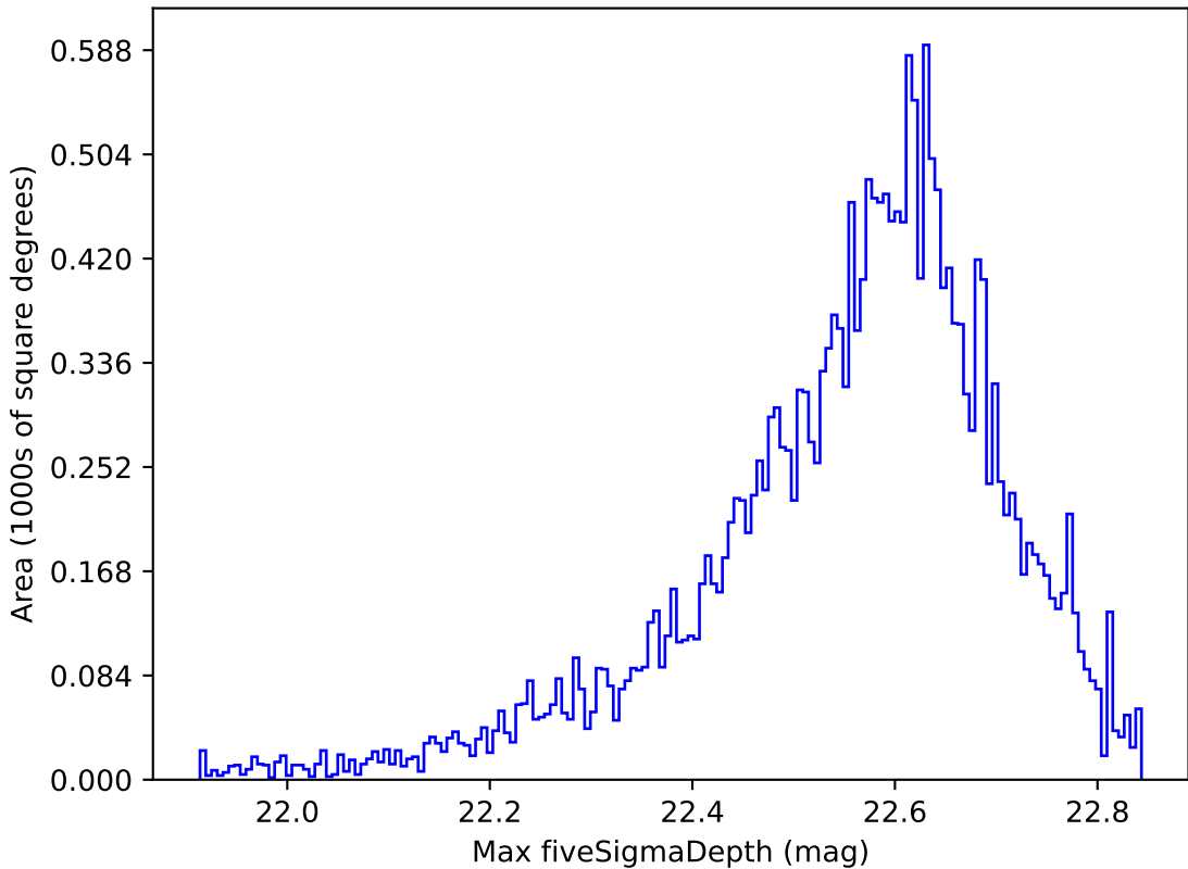
early_u_fpextra4.0_v3.4_10yrs All sky y band: Max fiveSigmaDepth
