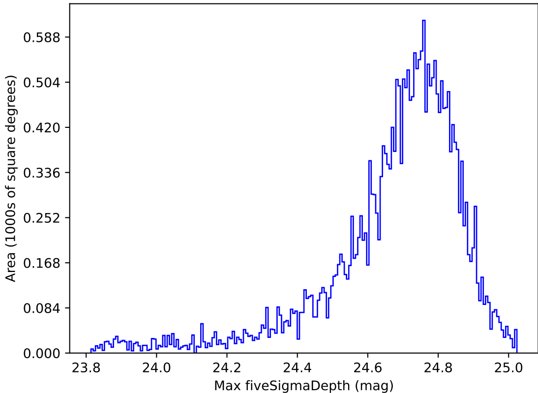
early_u_fpextra4.0_v3.4_10yrs All sky r band: Max fiveSigmaDepth
