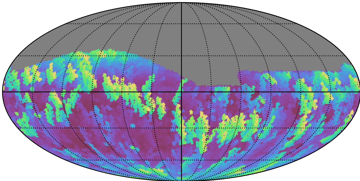
early_u_fpextra4.0_v3.4_10yrs Yr 1 z band: Max airmass
