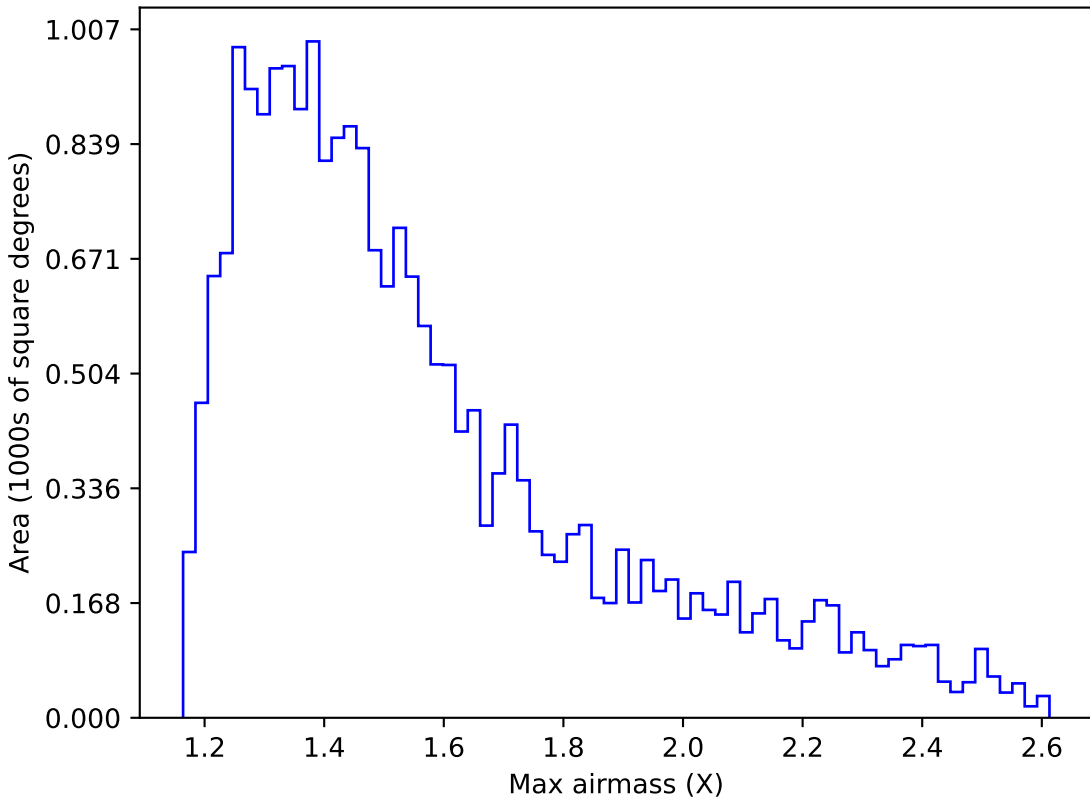
early_u_fpextra4.0_v3.4_10yrs Yr 1 y band: Max airmass
