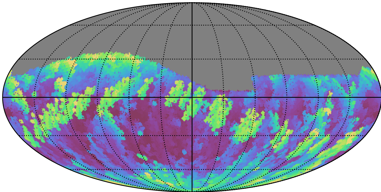
early_u_fpextra4.0_v3.4_10yrs Yr 1 r band: Max airmass
