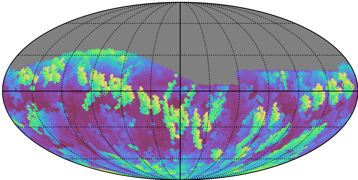
early_u_fpextra4.0_v3.4_10yrs Yr 1 i band: Max airmass
