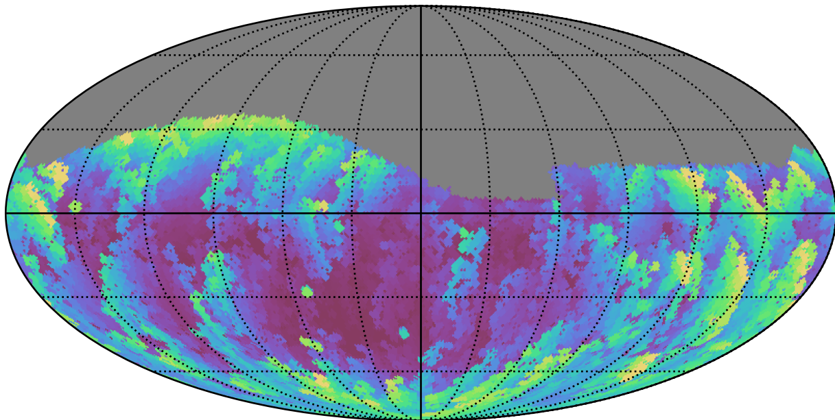
early_u_fpextra4.0_v3.4_10yrs Yr 1 g band: Max airmass
