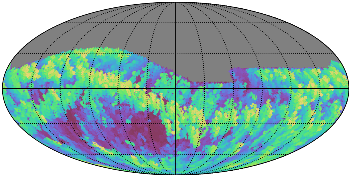
early_u_fpextra4.0_v3.4_10yrs Yr 1 all bands: Max airmass
