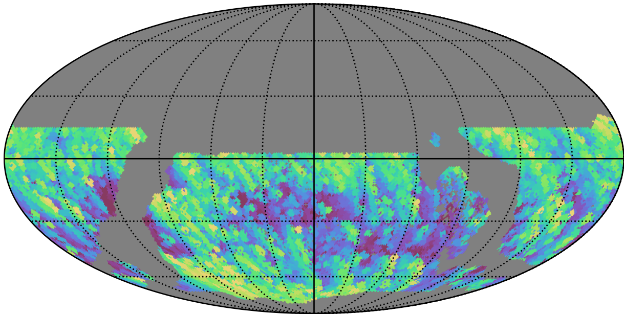
early_u_fpextra4.0_v3.4_10yrs WFD y band: Max airmass
