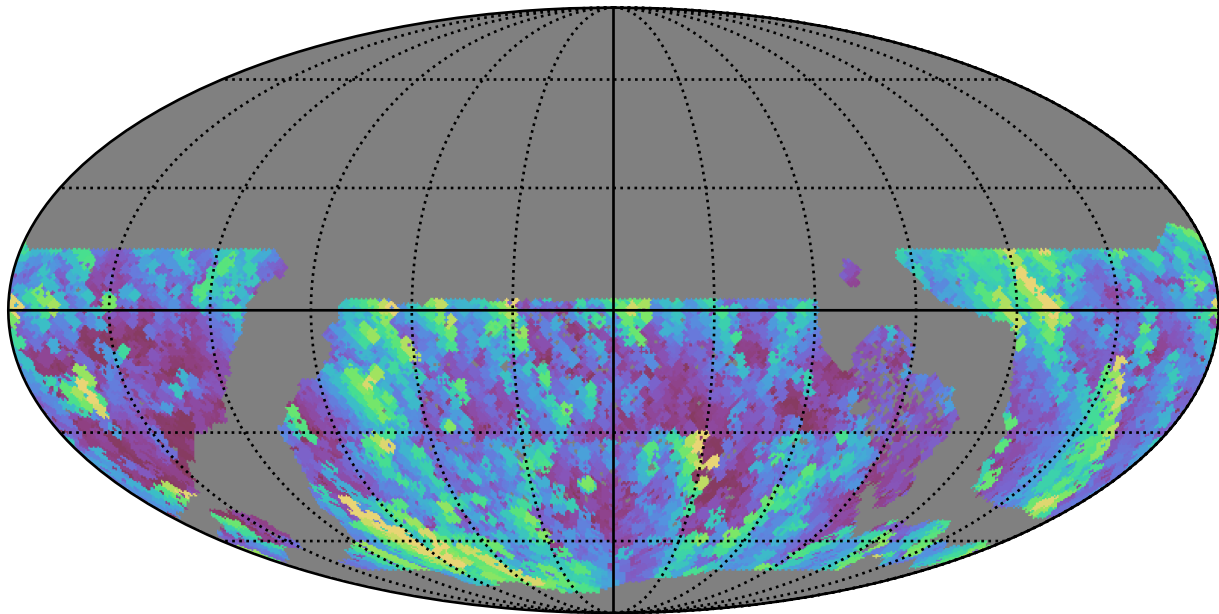
early_u_fpextra4.0_v3.4_10yrs WFD u band: Max airmass
