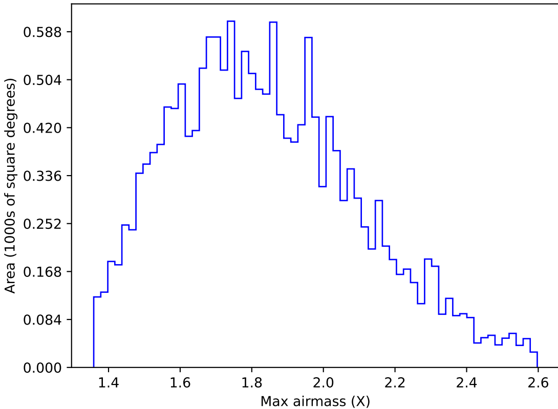
early_u_fpextra4.0_v3.4_10yrs WFD u band: Max airmass
