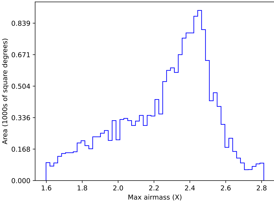
early_u_fpextra4.0_v3.4_10yrs WFD r band: Max airmass
