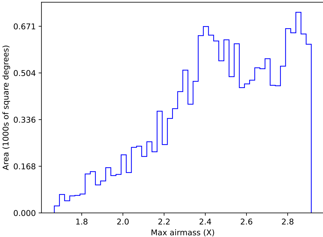
early_u_fpextra4.0_v3.4_10yrs WFD i band: Max airmass
